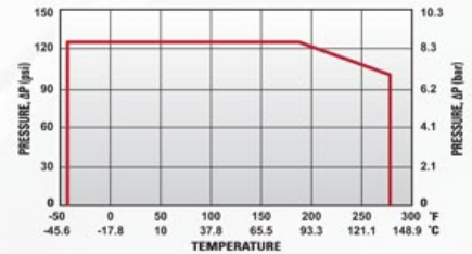
60PS Series Temperature
