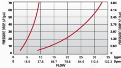
60PS Series Water Flow
